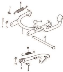
Fig.29 CAVALETES (T06-S270-0006) REF.No.
