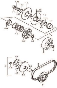
Fig.16 TRANSMISSAO (1) (T06-S153-0012) REF.No.
